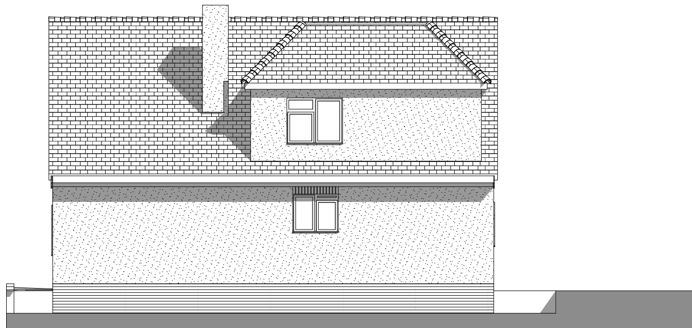
North East Elevation as Existing
