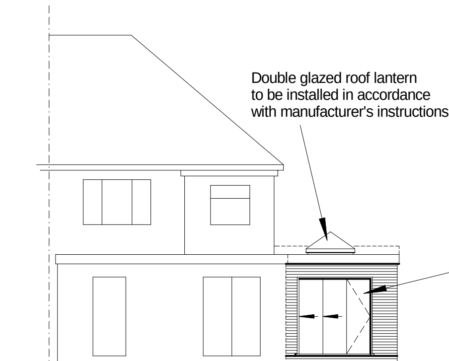
REAR
