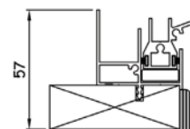
Cill Detail
