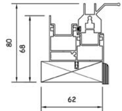
Cill Detail
