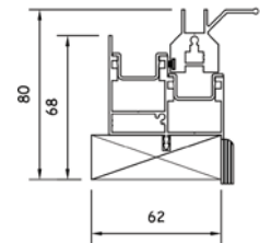
Cill Detail
