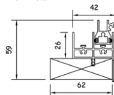
Cill Detail
