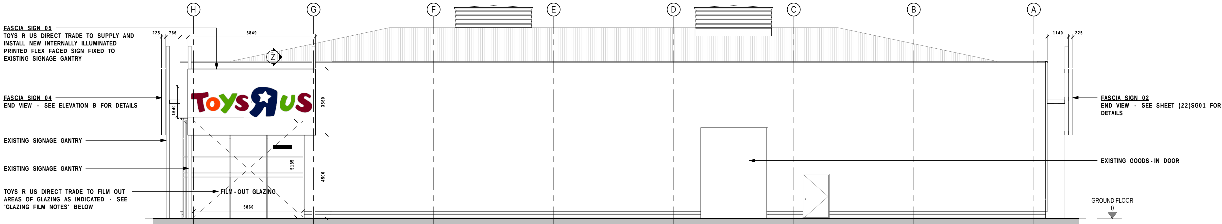
ELEVATION C
