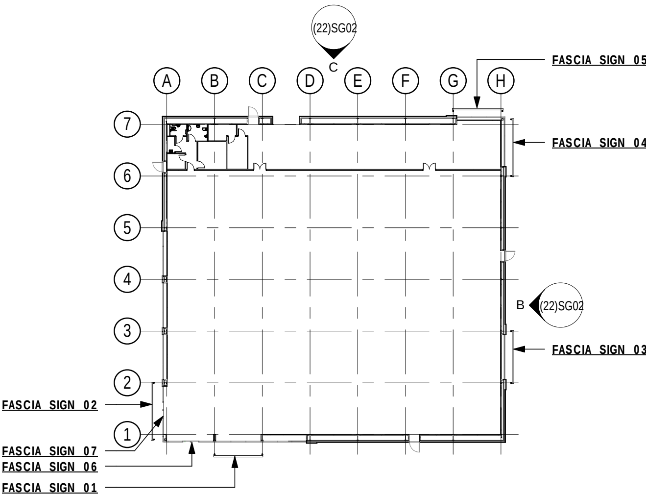
KEY PLAN
