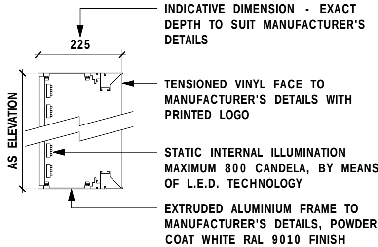
SECTION Z
