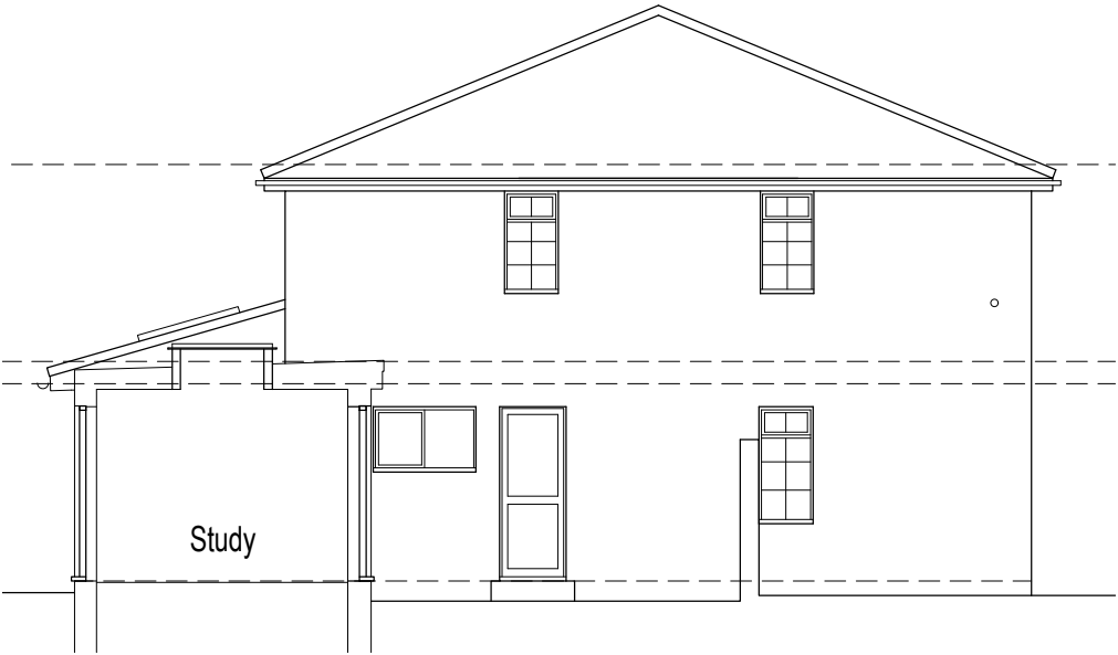
South Elevation/ Section
