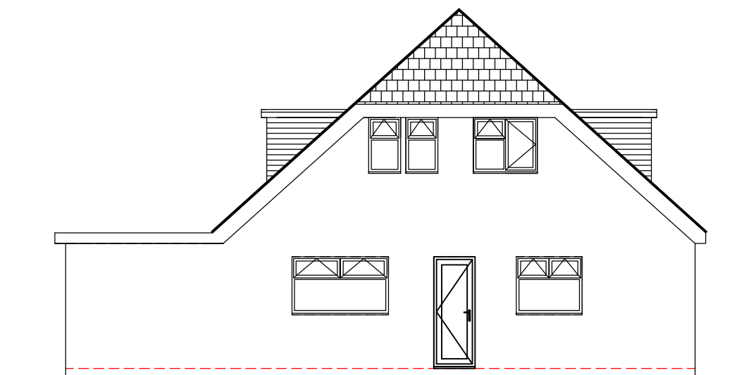
Existing Right elevation
