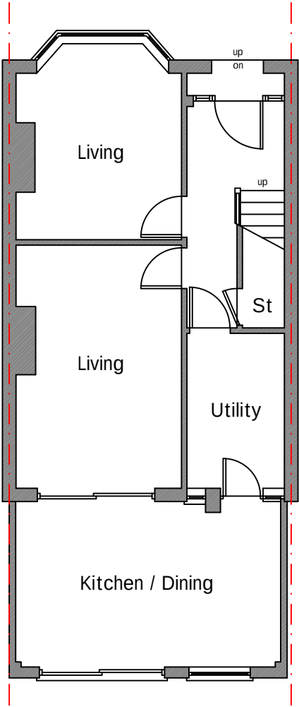
Ground Floor Layout
