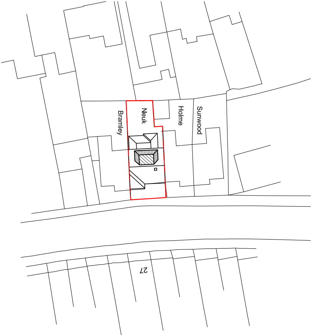
Crown Copyright. All rights reserved. Licence no. 100019980 PROPOSED BLOCK PLAN SCALE 1-500 0 10 20 30 Metres NORTH
