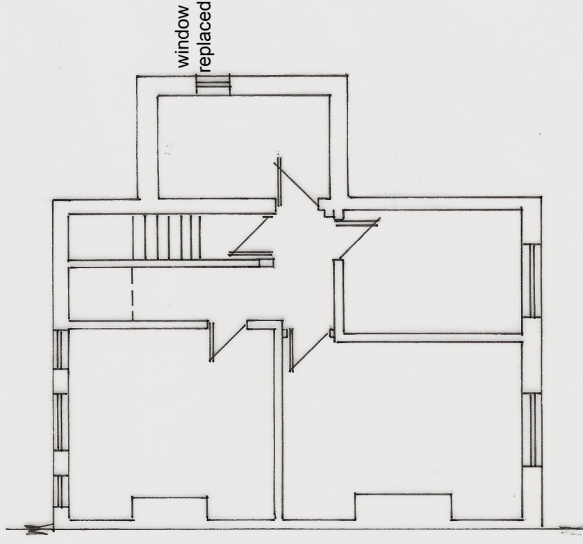
lower ground floor plan
