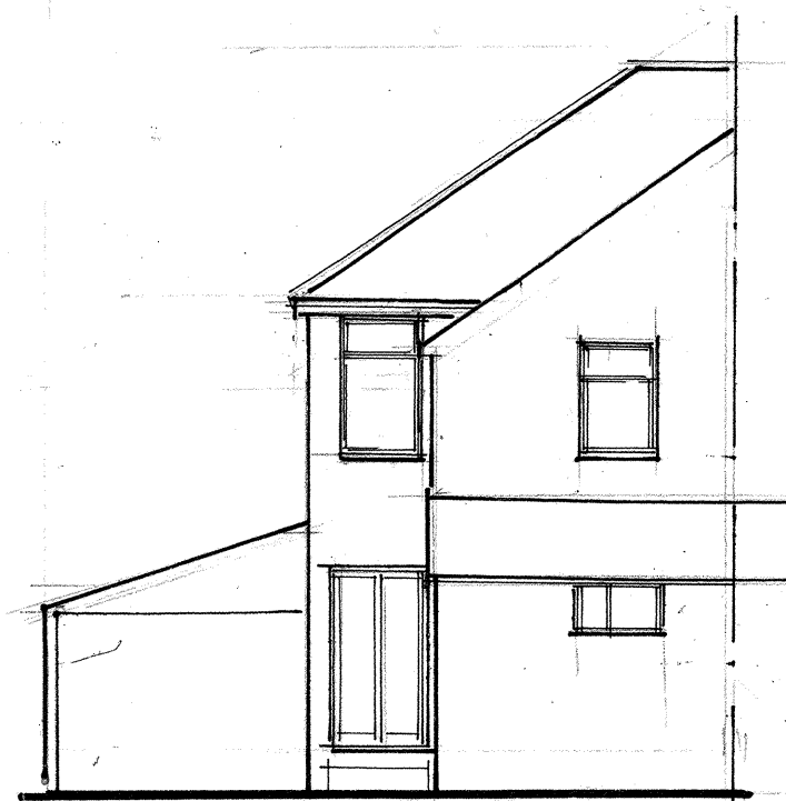
EAST ELEVATION
