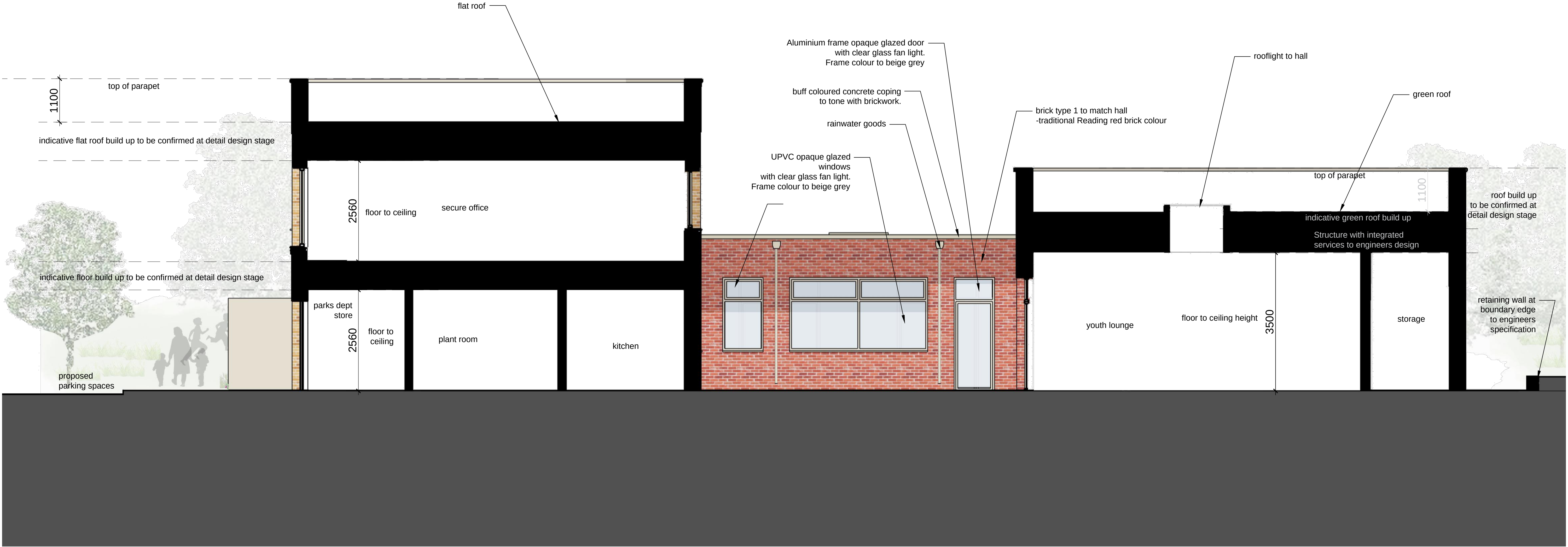
1 Section CC Scale 1:100 @A3
