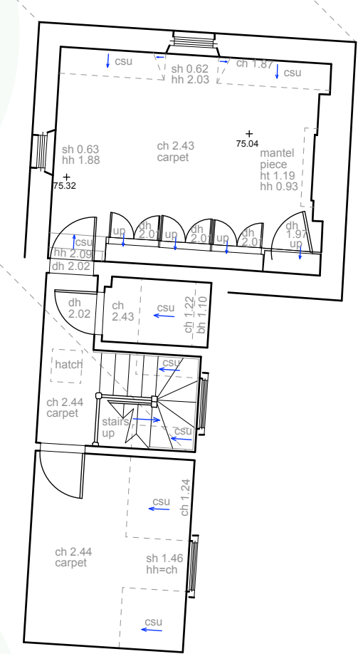
EXISTING ATTIC PLAN
