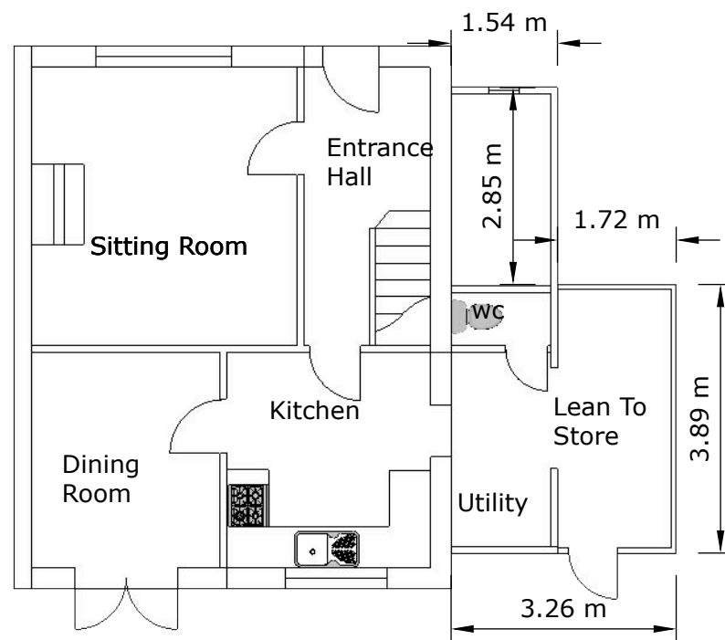
Existing Ground Floor layout Scale: 1/100 @ A3
