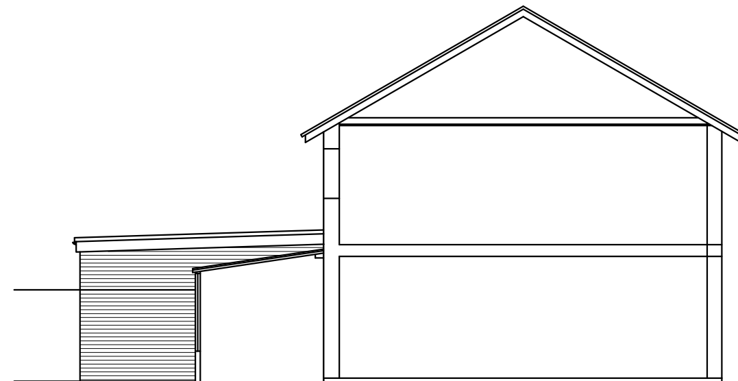
SIDE - proposed (from No 45)
