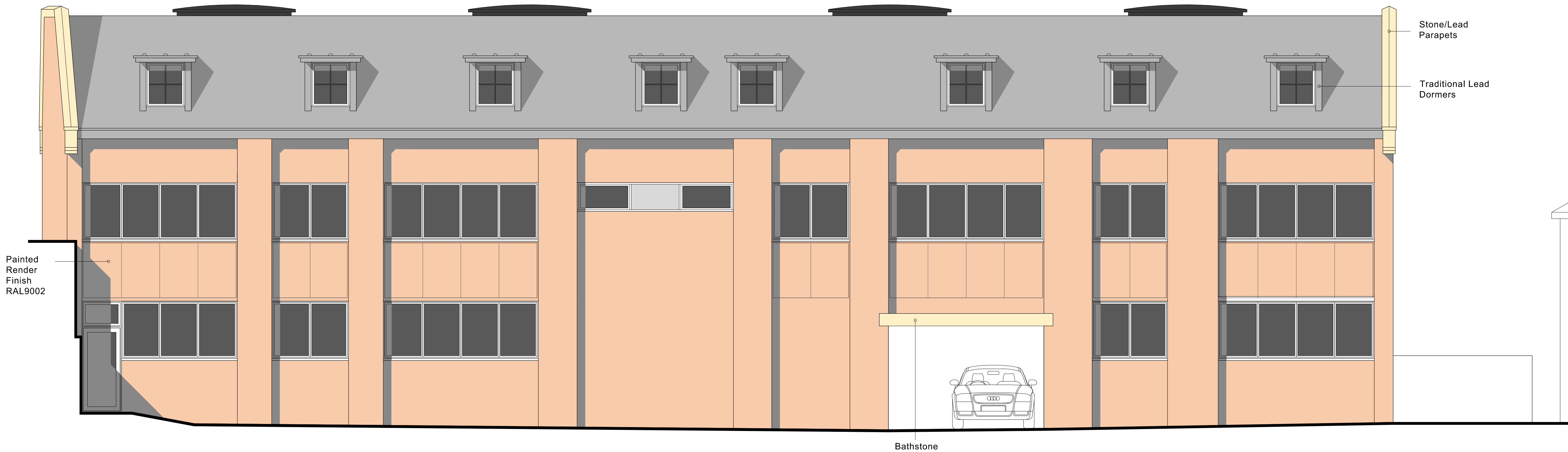
West Elevation
