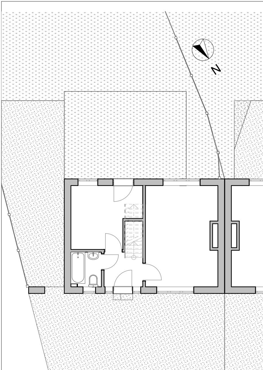
1 - GF-Ground Floor as Existing 1:100
