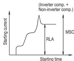
The relationship between the starting time and the starting current
