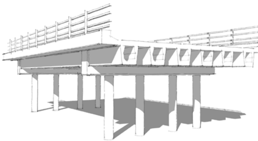
Figure 66. Baseline viaduct with concrete girder, four column support and square edge soffit
