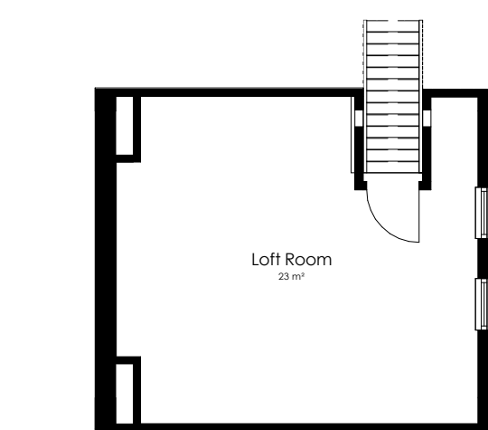
Existing Loft Level 1:100
