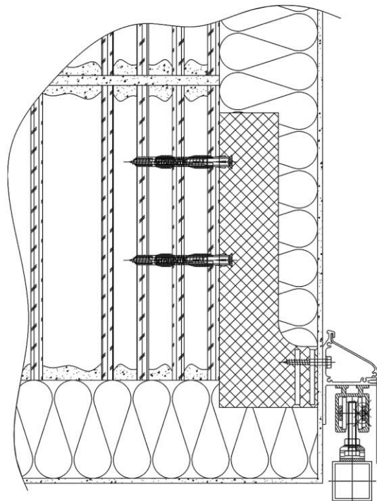
Supporting bracket
