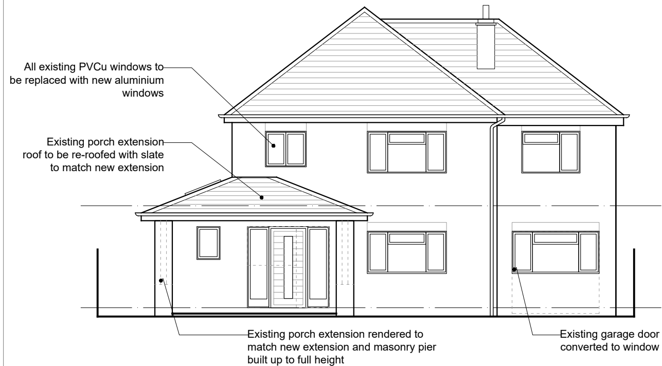
FRONT ELEVATION
