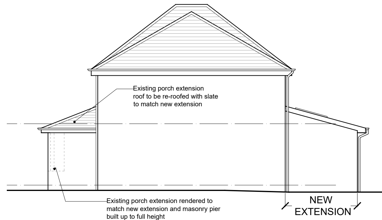
SIDE ELEVATION
