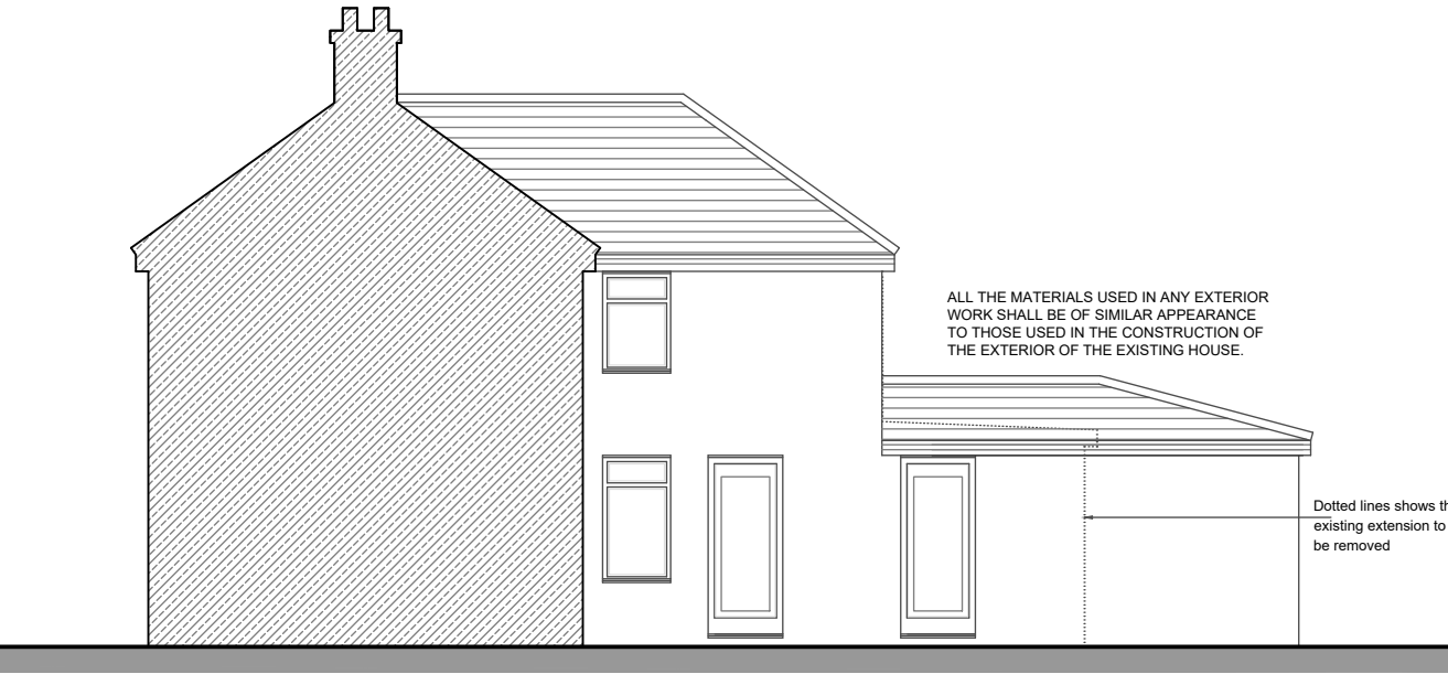
REAR (SSW) ELEVATION AS PROPOSED 2 CALLINGTON ROAD, READING - RG2 7QJ
