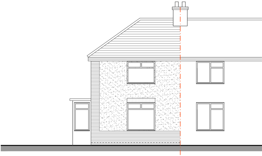
SIDE (WNW) ELEVATION AS PROPOSED 2 CALLINGTON ROAD, READING - RG2 7QJ
