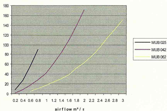
Pressure Loss Graph
