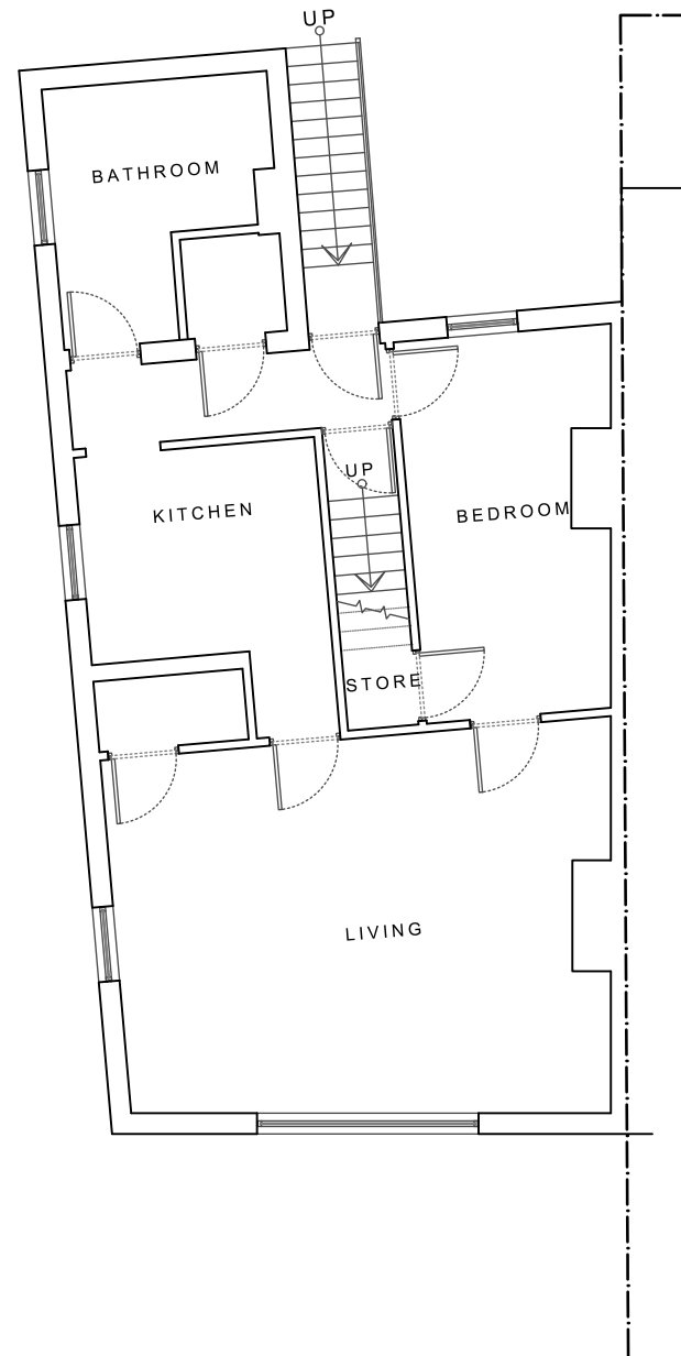
FIRST FLOOR PLAN AS EXISTING 576 OXFORD ROAD, READING- RG30 1EG
