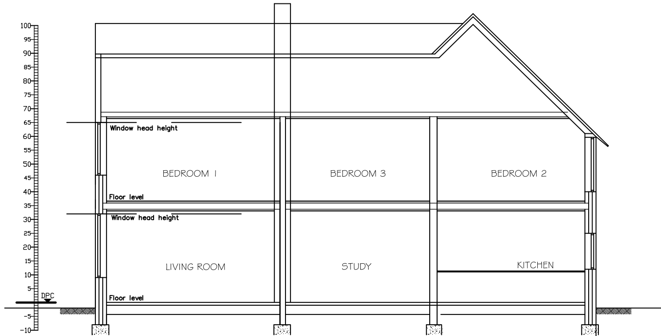
TYPICAL SECTION 1/100 40 HARROGATE RD
