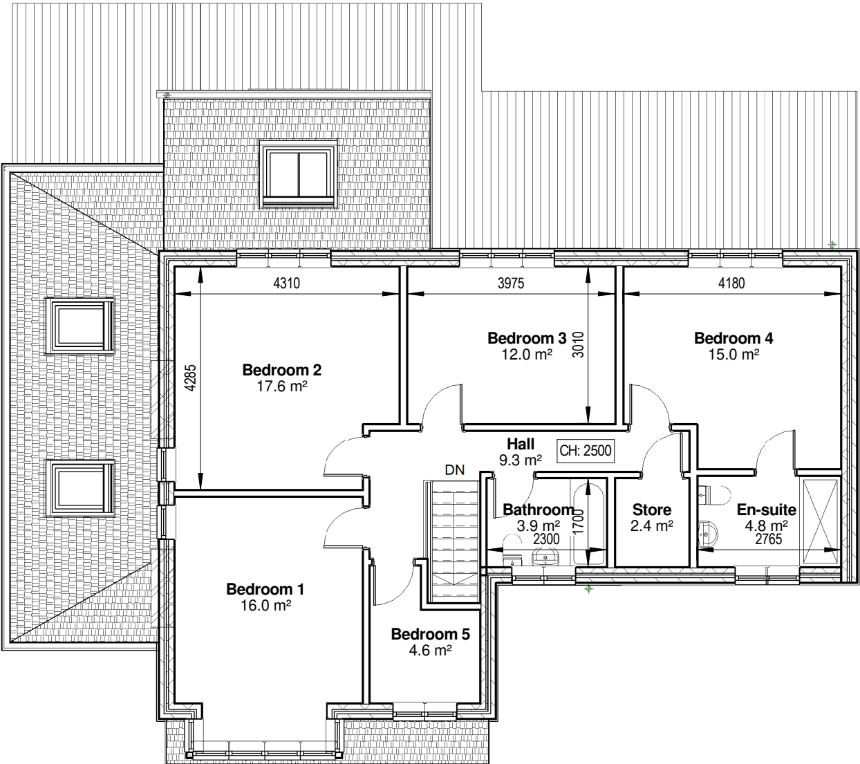
2 02. First floor plan 1 : 100
