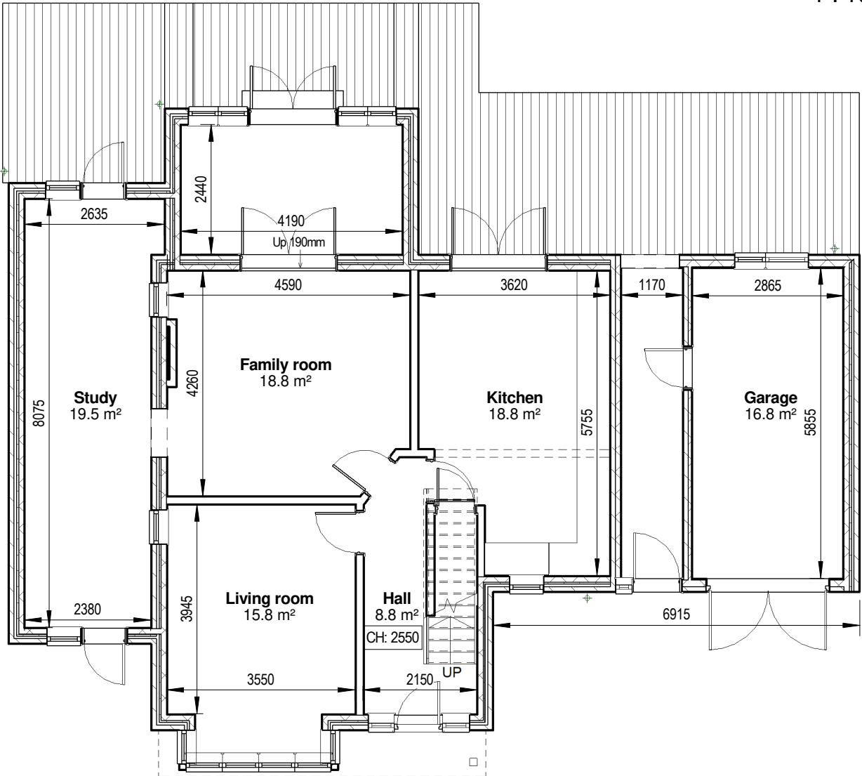
1 01. Ground floor plan 1 : 100
