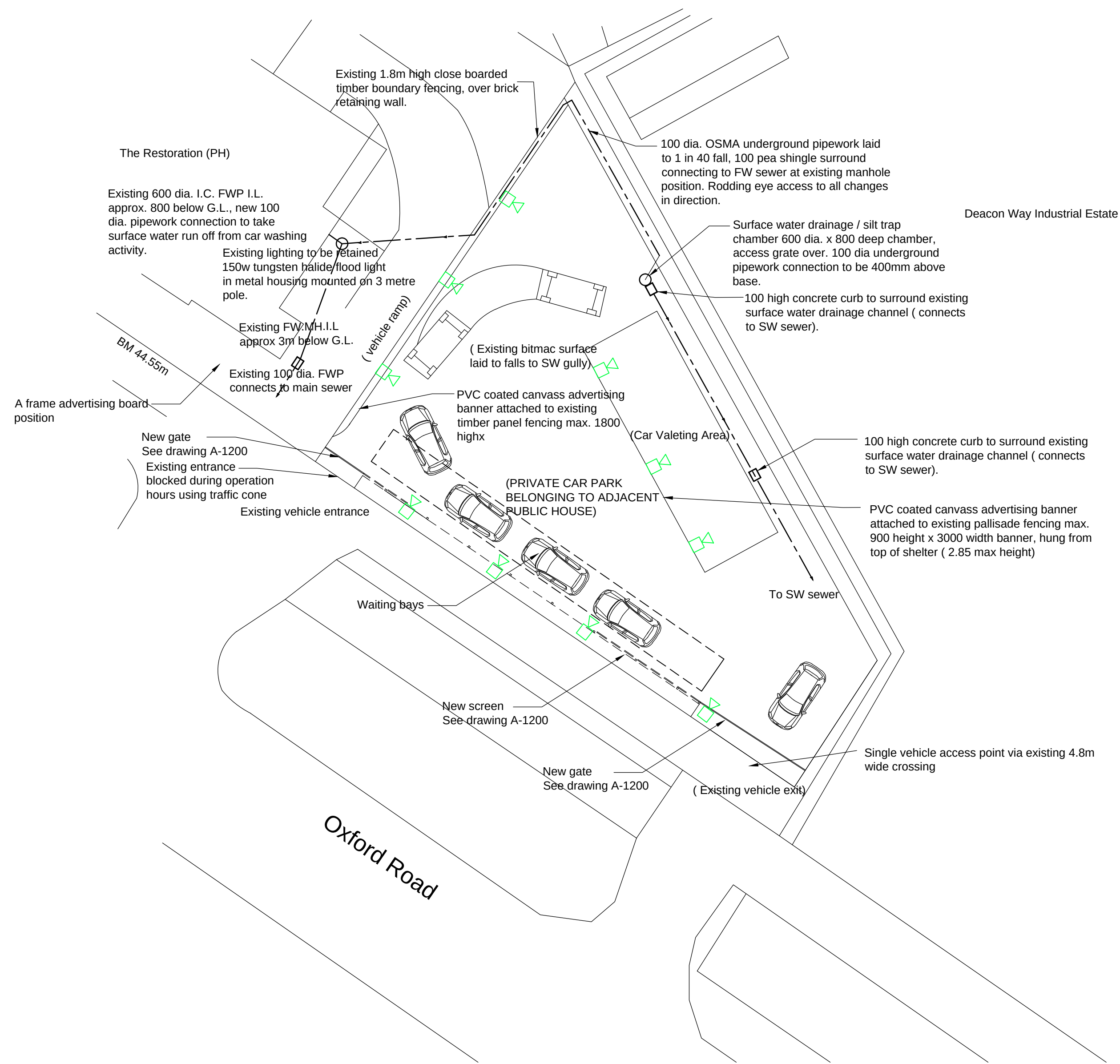
CARWASH PLAN 1:200 @ A1
