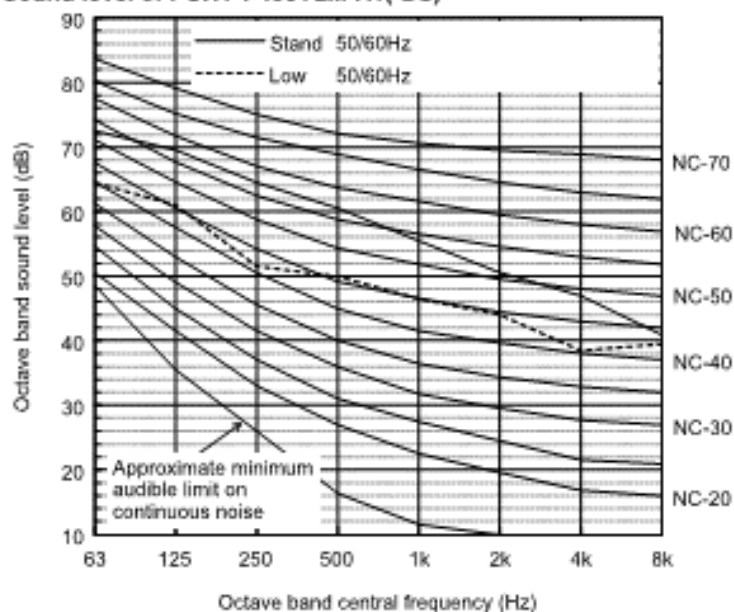
Sound level of PURY-P450YLM-A1(-BS)
