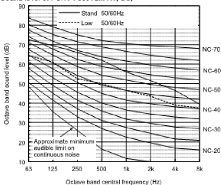
Sound level of PURY-P500YLM-A1(-BS)
