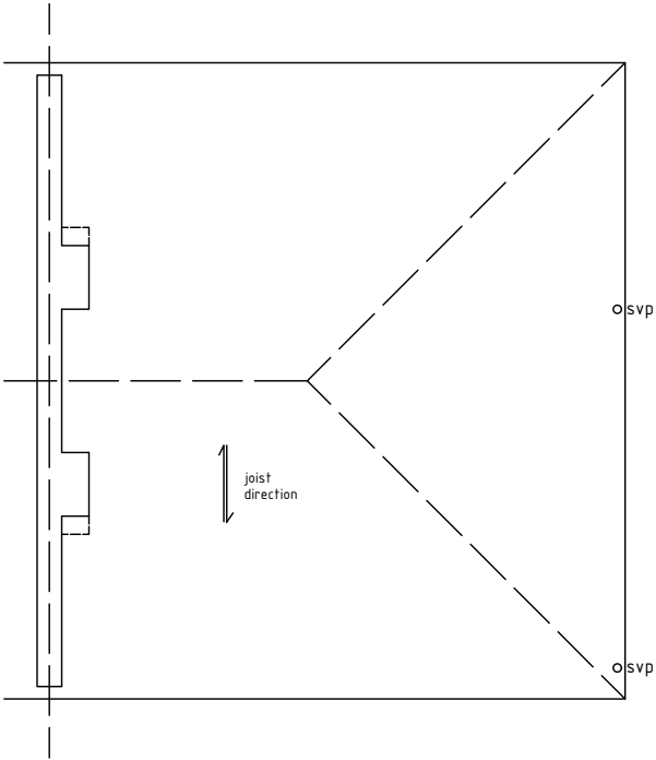
ROOF PLAN
