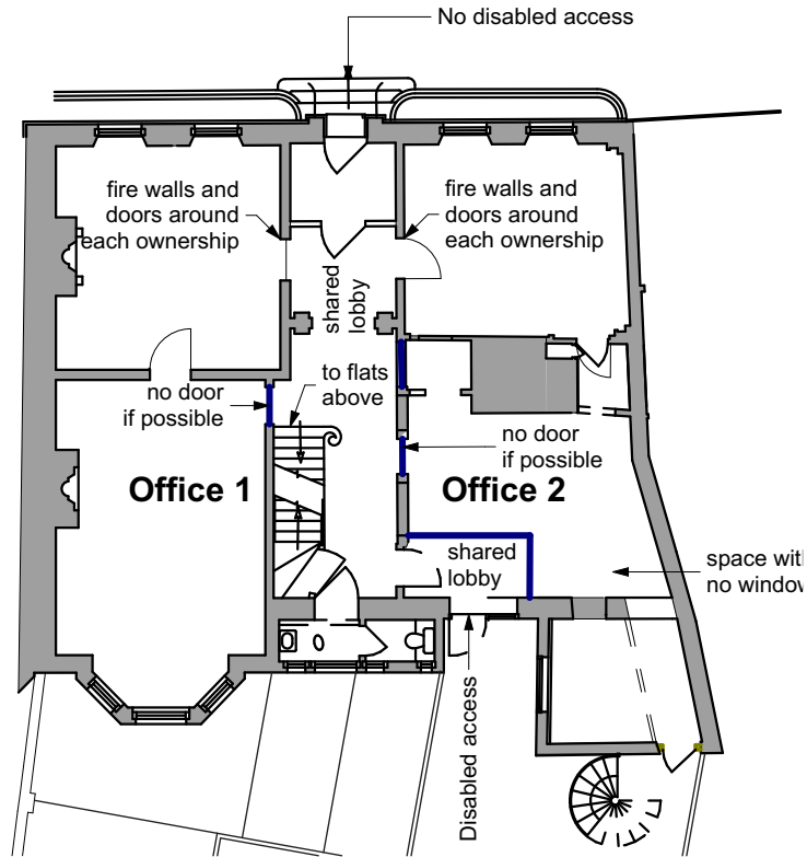
Ground Floor Plan 1:200
