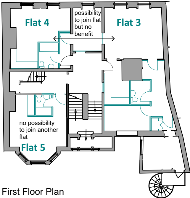
First Floor Plan 1:200
