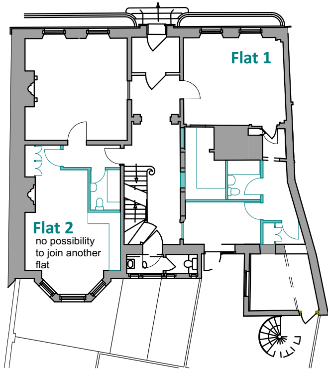
Ground Floor Plan 1:200
