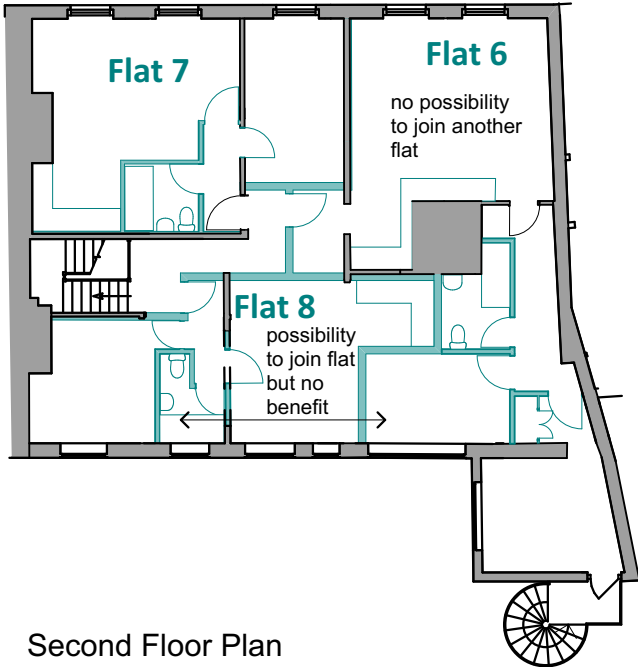
Second Floor Plan 1:200
