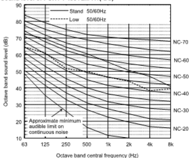
Sound level of PURY-P450YLM-A1(-BS)
