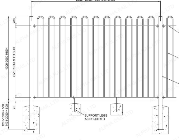
BOW TOP RAILING DETAIL
