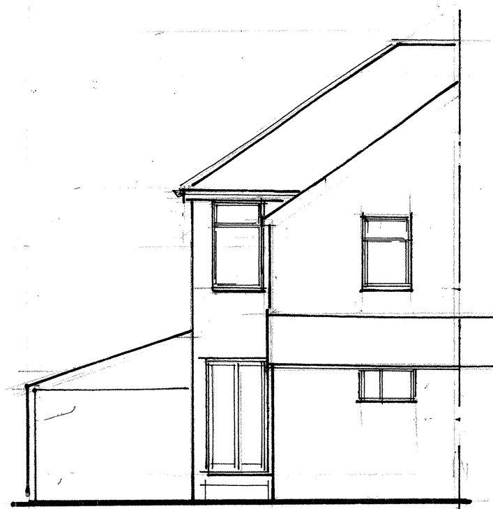
EAST ELEVATION
