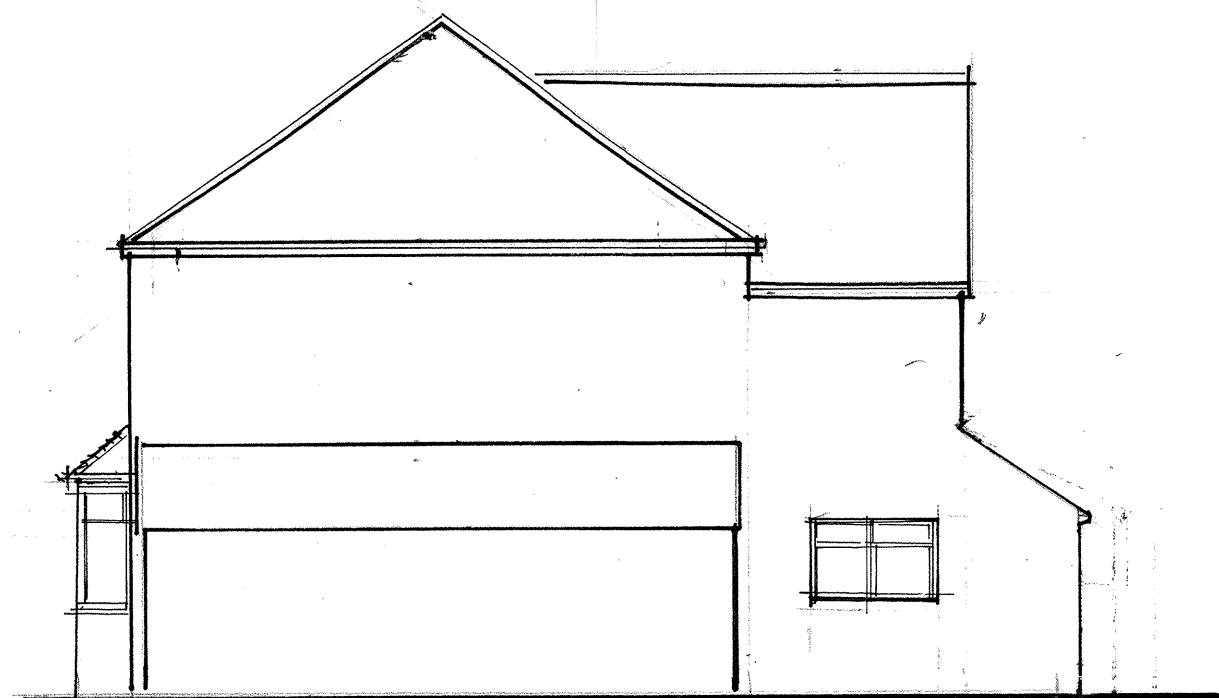
SOUTH ELEVATION
