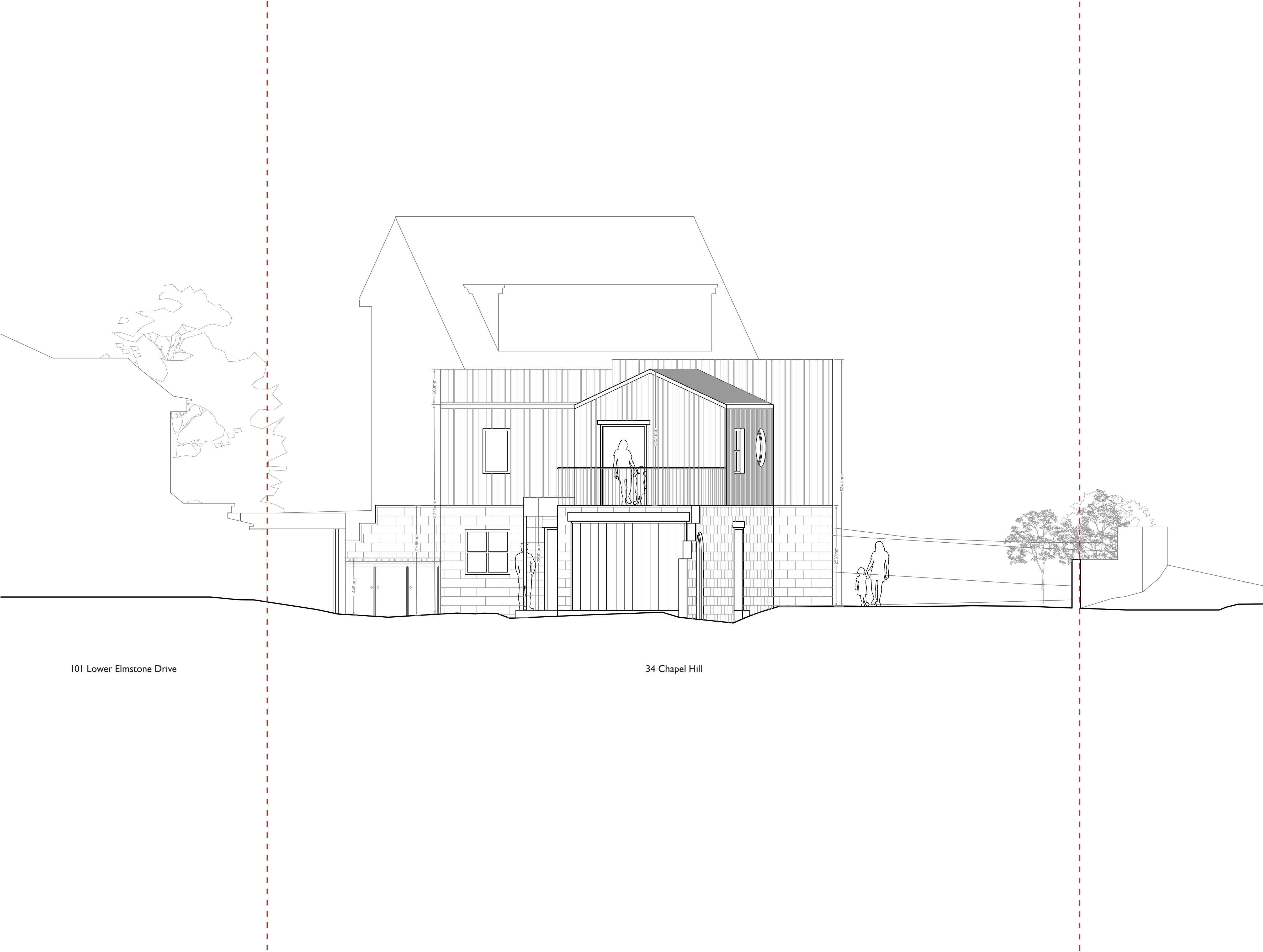
Proposed Side (West) Elevation C
