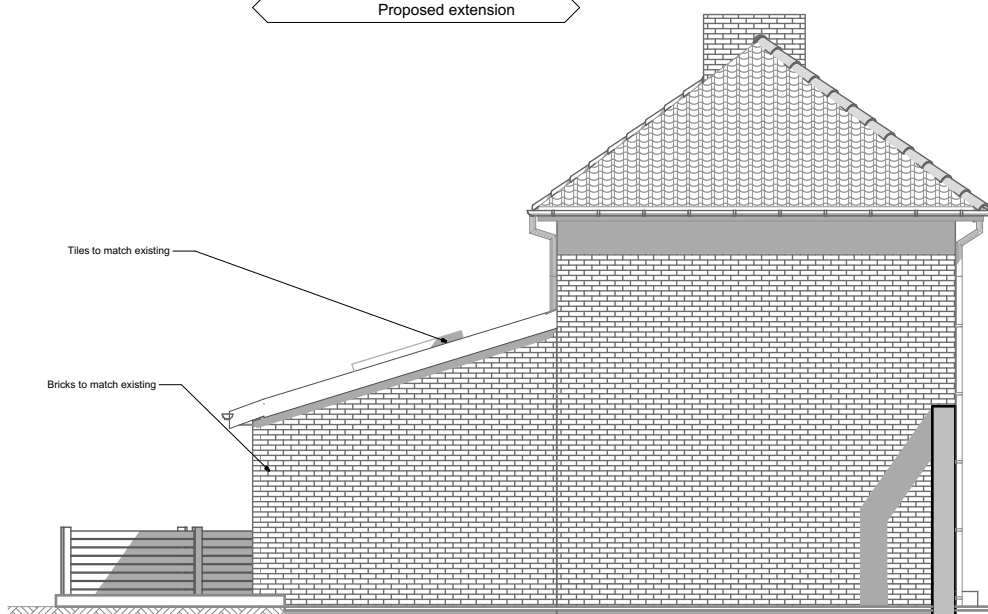
South East Elevation - Proposed 1:100
