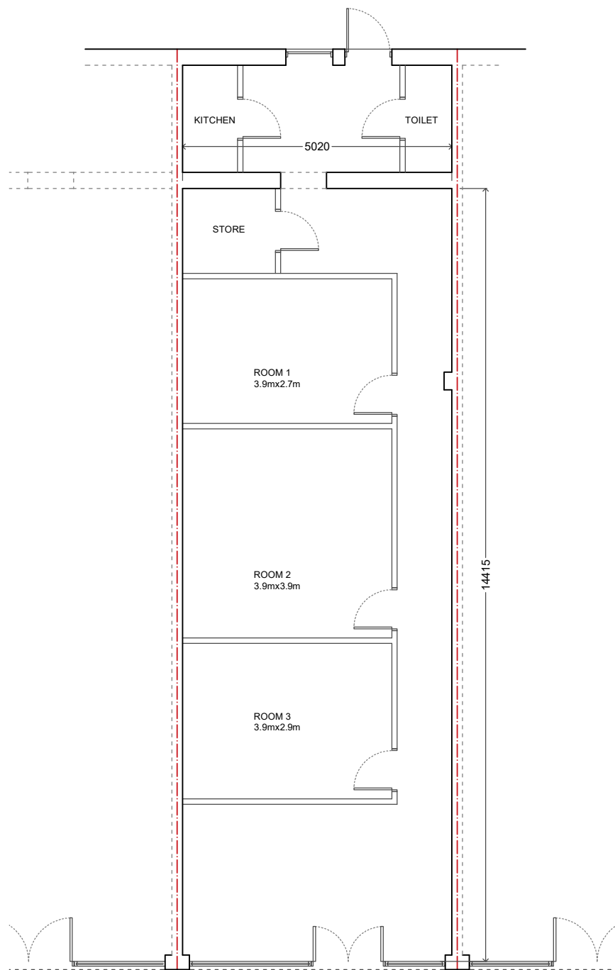
GROUND FLOOR PLAN AS EXISTING UNIT 45, MEADWAY PRECINCT, TILEHURST, READING - RG30 4AA
