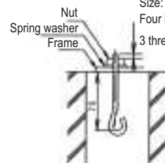
Foundation bolt executing method
