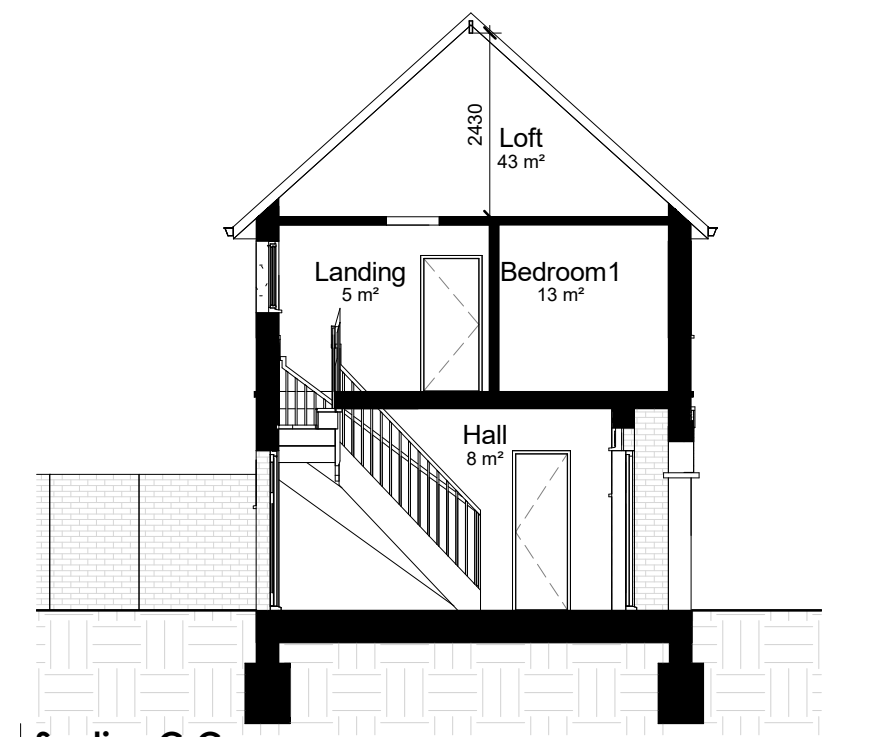
Section C-C
