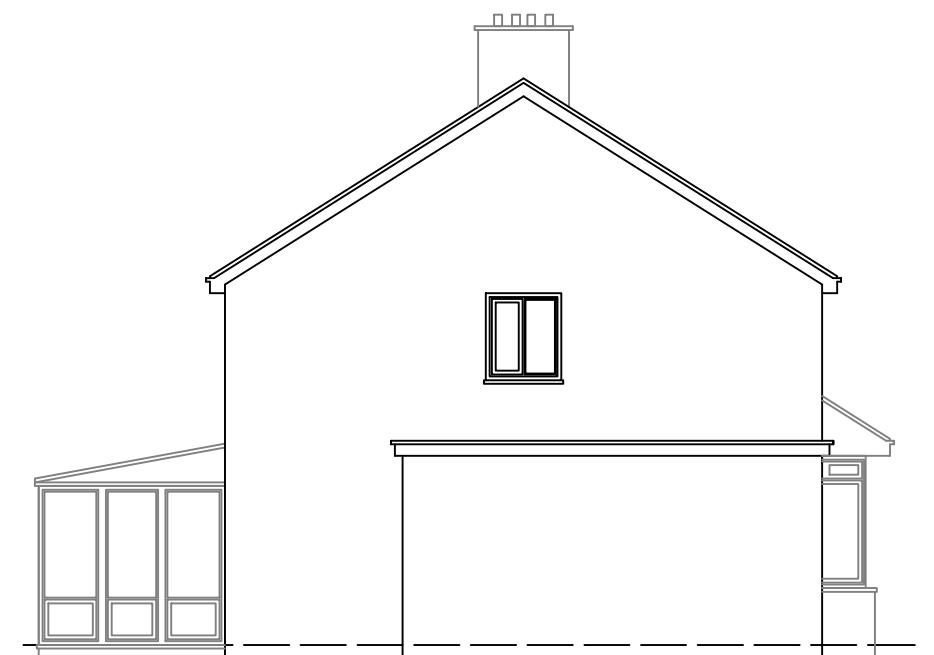
EXISTING SIDE-2 ELEVATION
