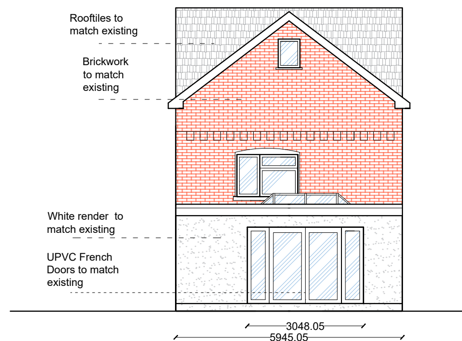
Rear Elevation
