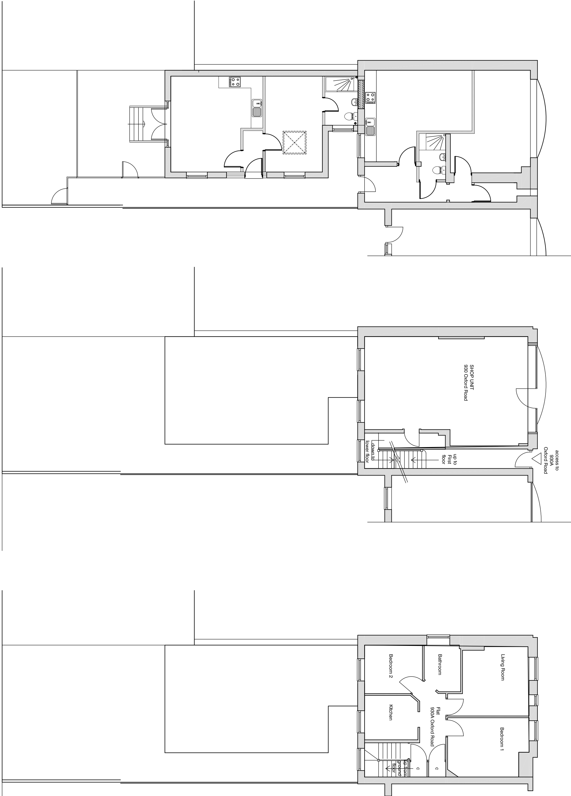
Lower Ground Floor Plan [garden level] EXISTING 1:100
