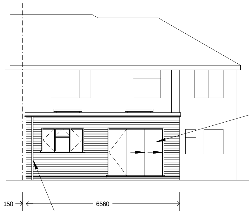
REAR
