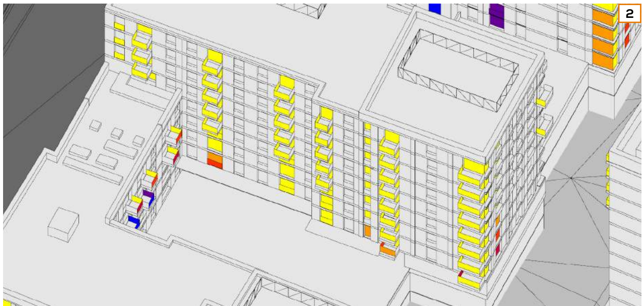
Fig. 40: Winter Probable Sunlight Hours - View 2
