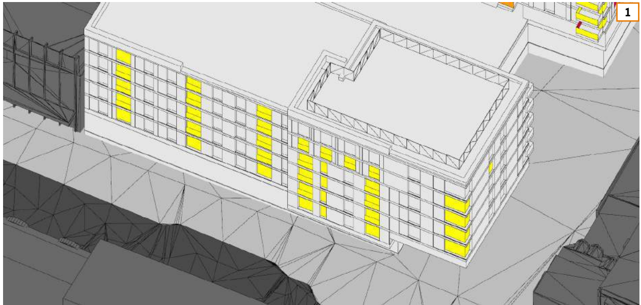
Fig. 39: Winter Probable Sunlight Hours - View 1
