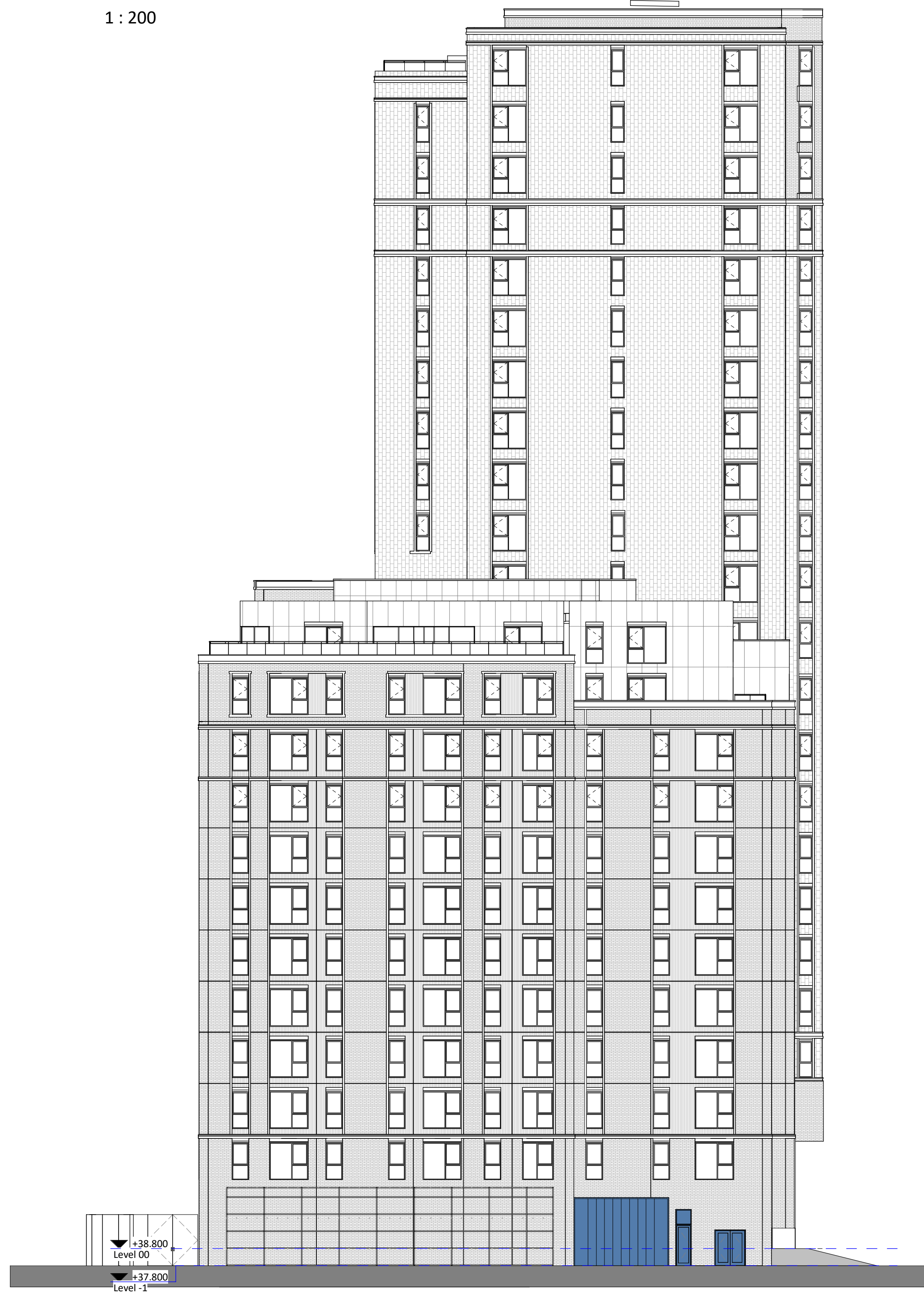
East Elevation 1 : 200
