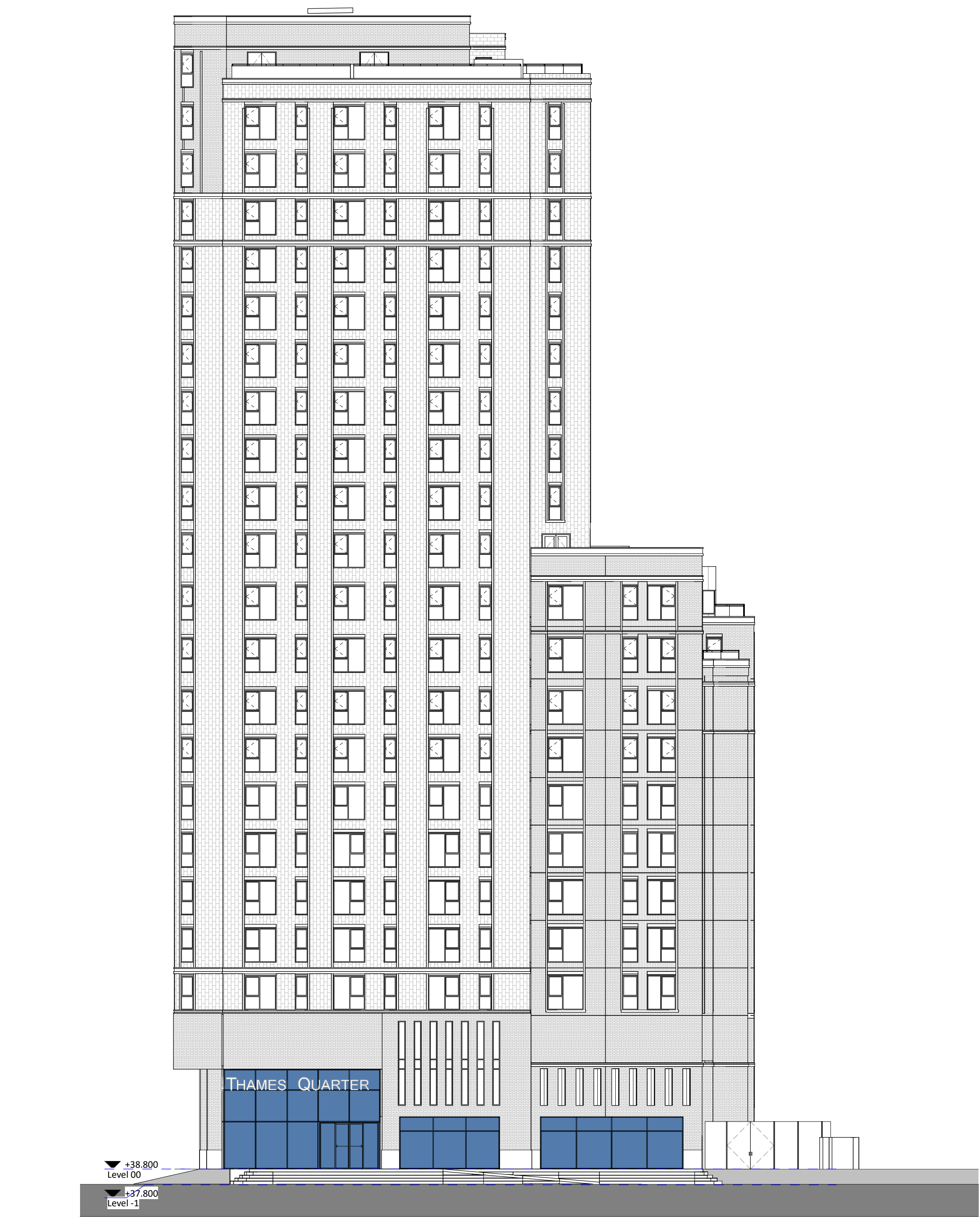
West Elevation 1 : 200
