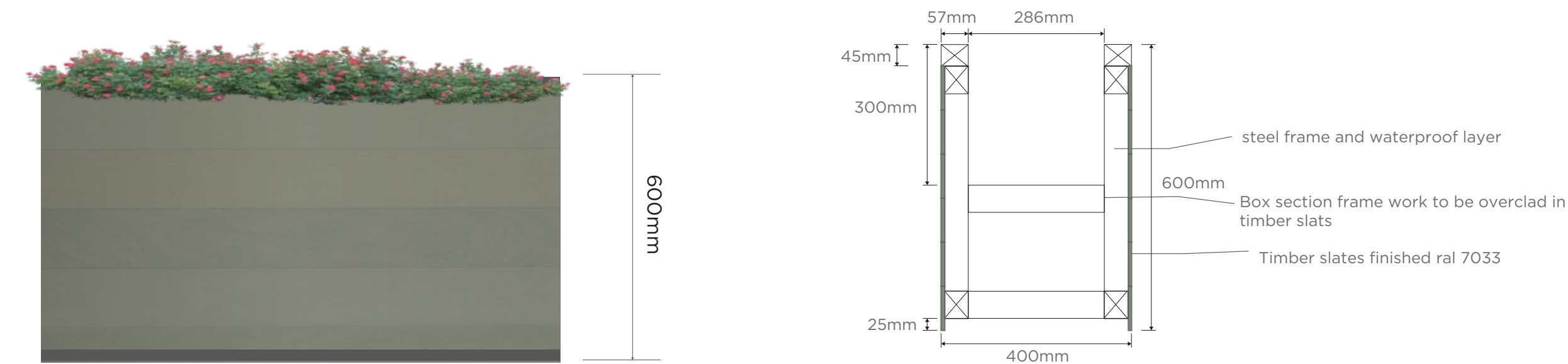
Signage 4: Planter wooden box with foliage. Finished Ral 7033 Cement Grey
