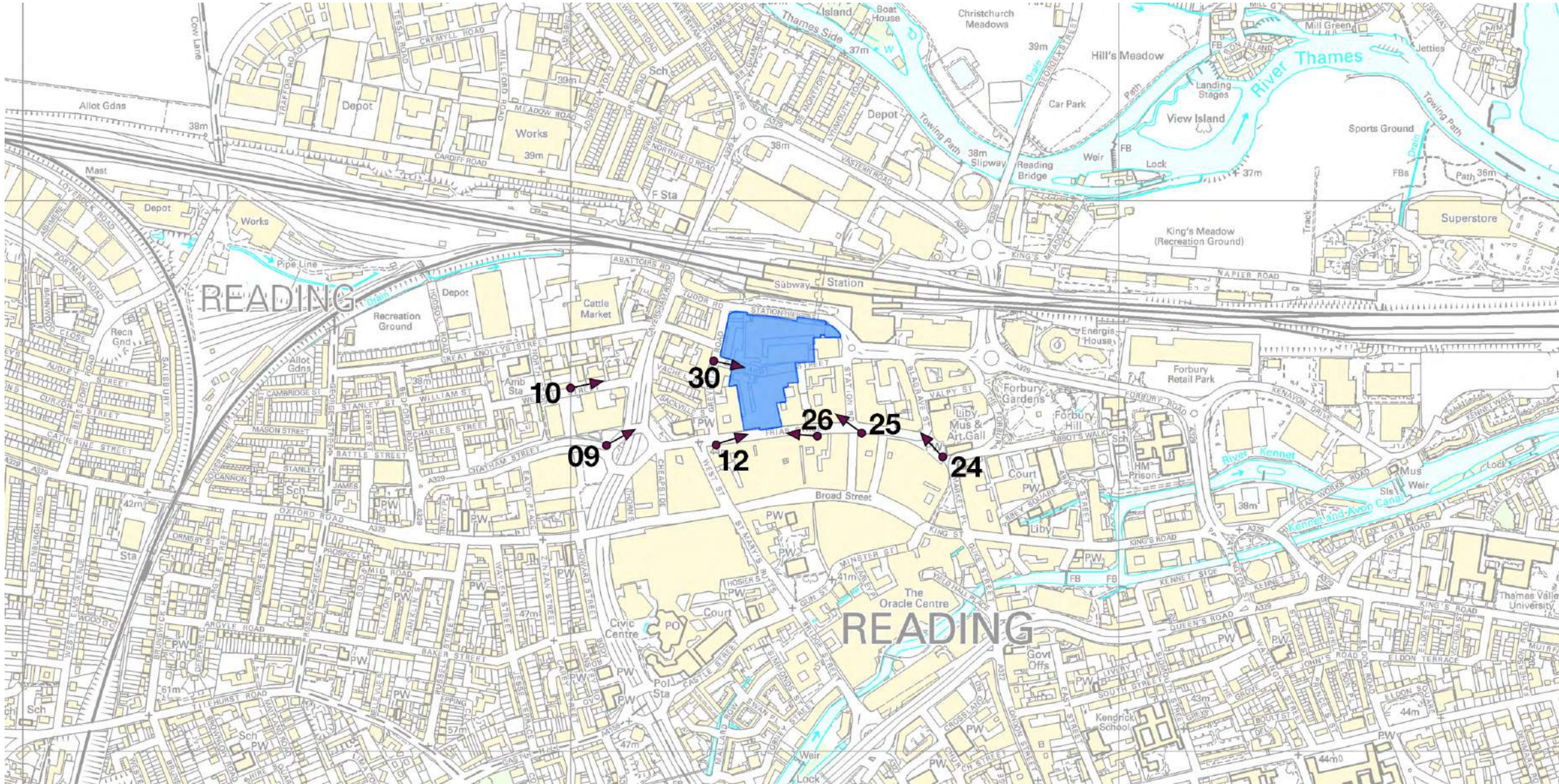
Views map
