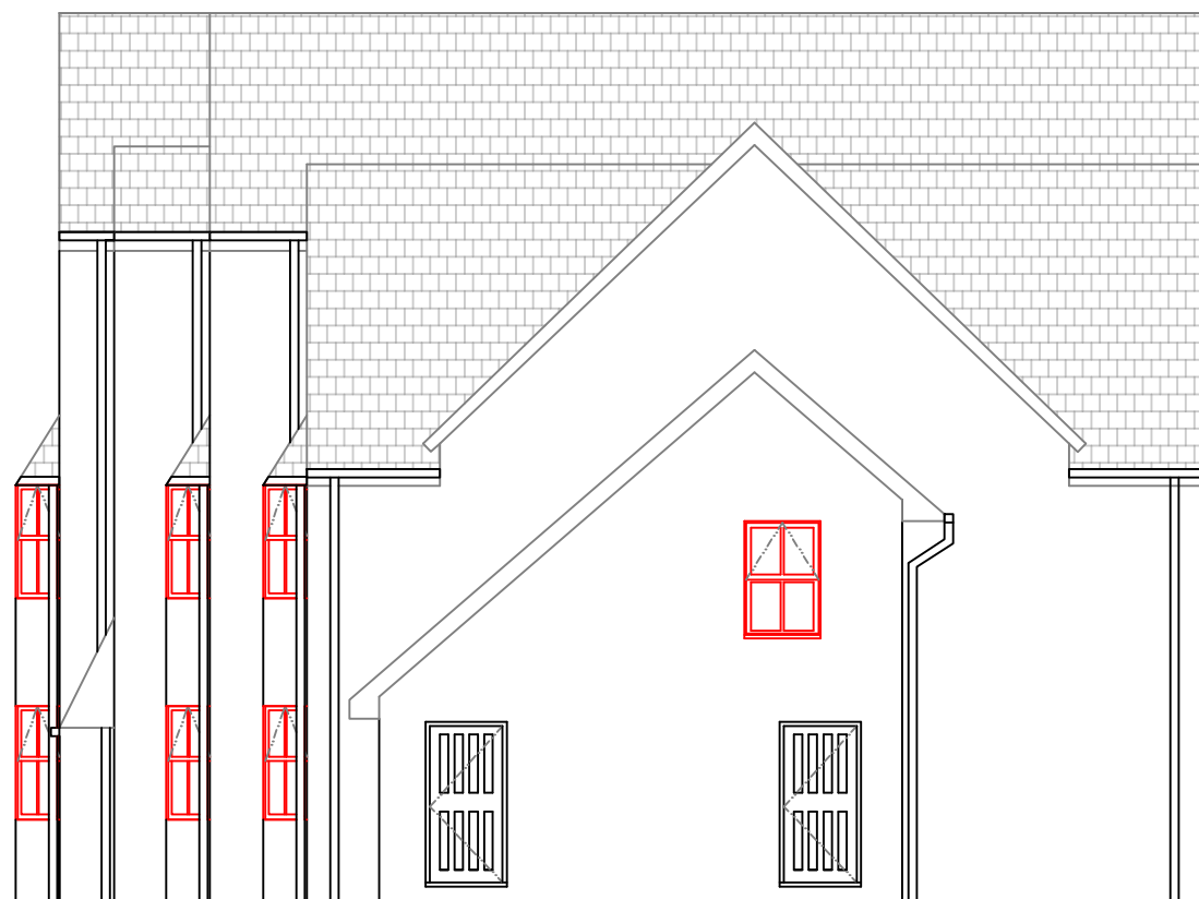
9-16 Simone House Proposed Elevation View B 1:100
