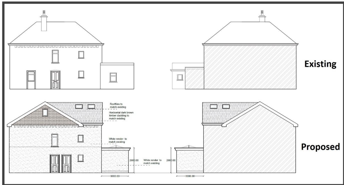
6. Existing and proposed side elevations
