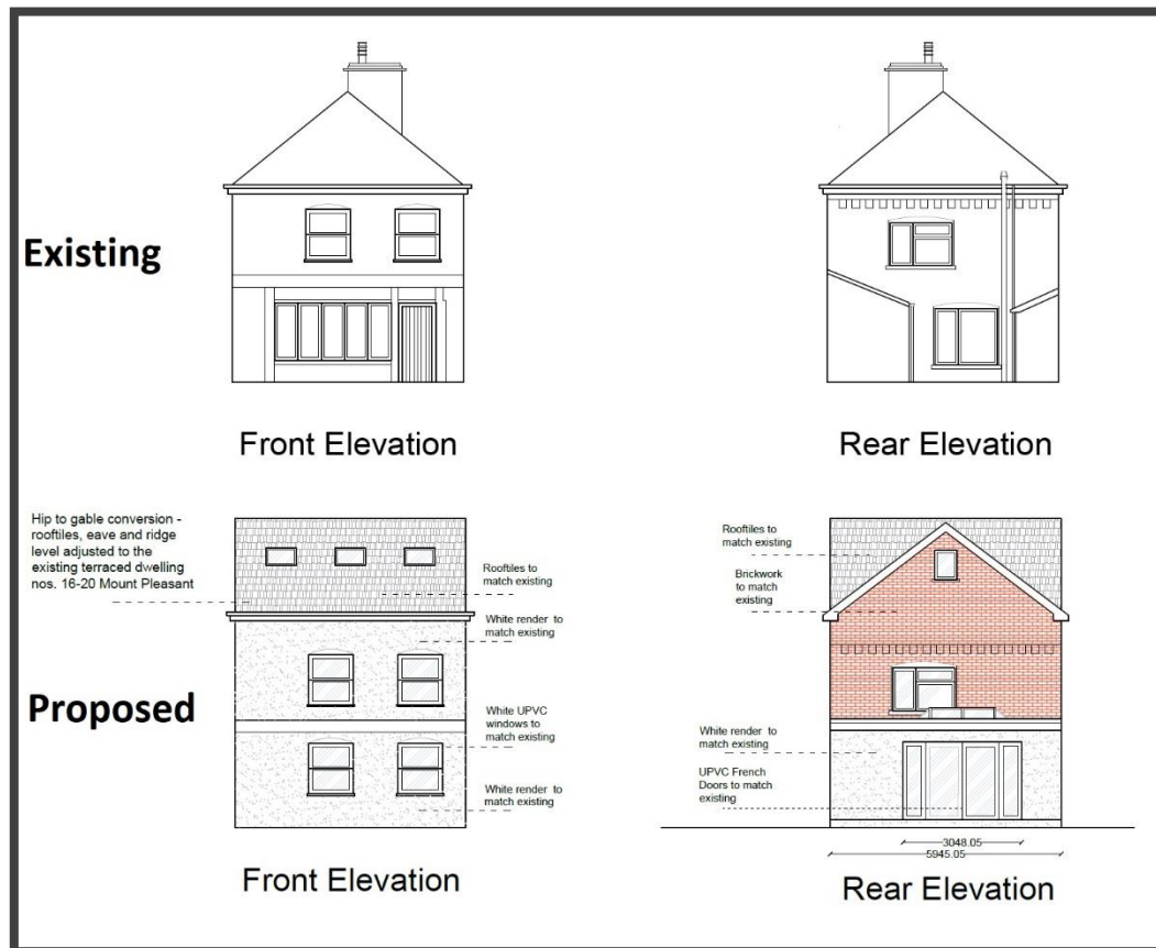
7. Existing and proposed front and rear elevation
