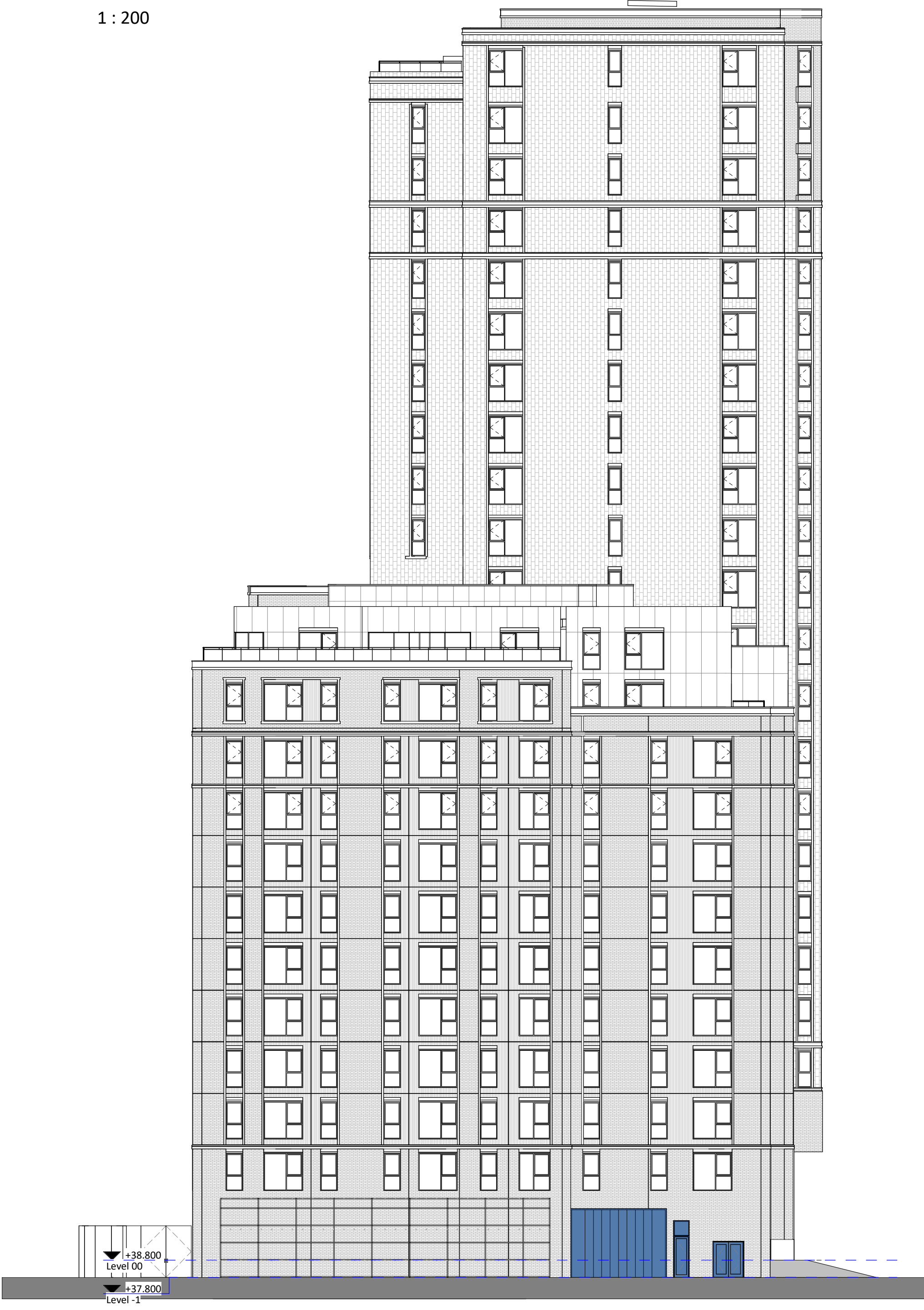
East Elevation 1 : 200
