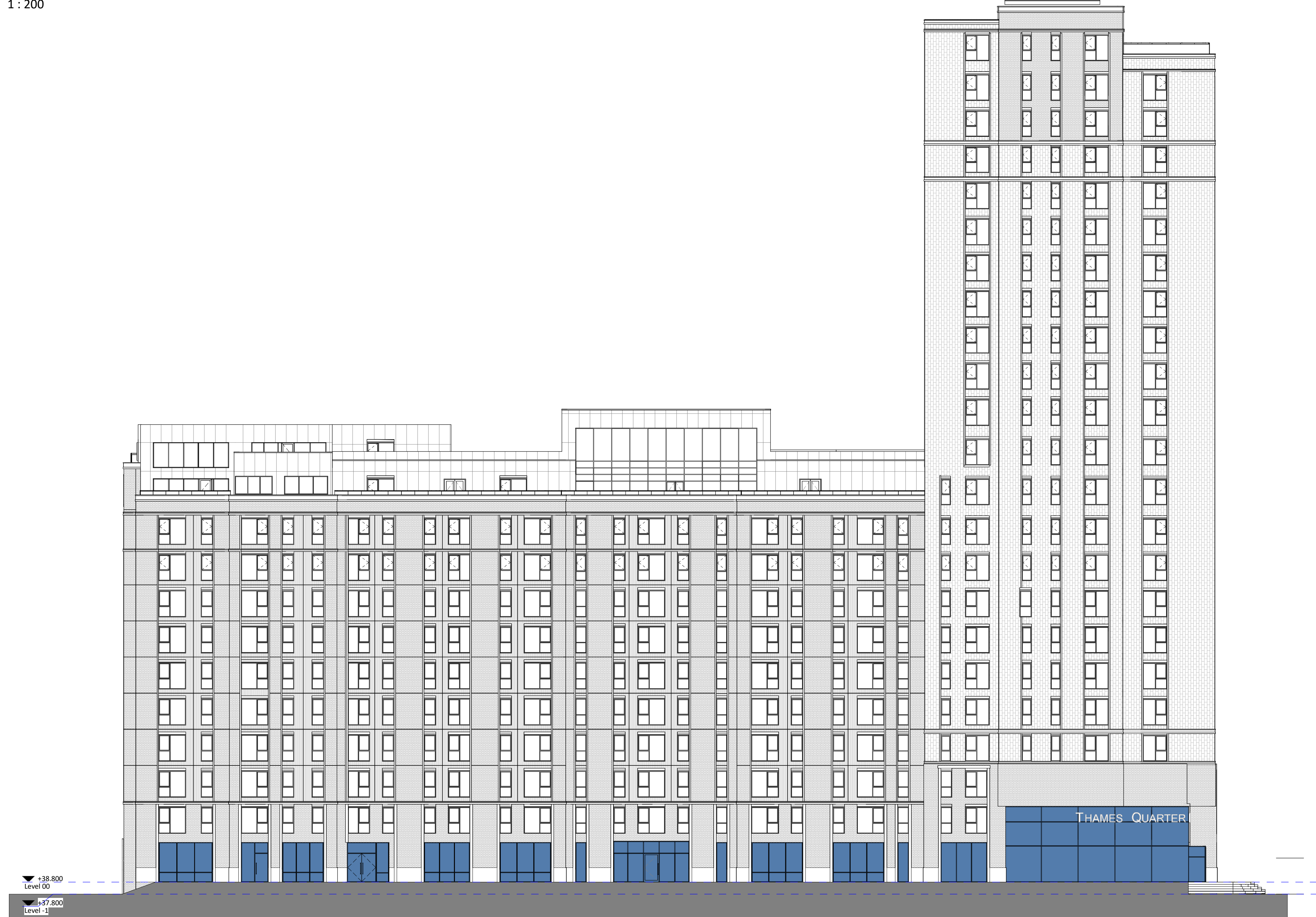
North Elevation 1 : 200
