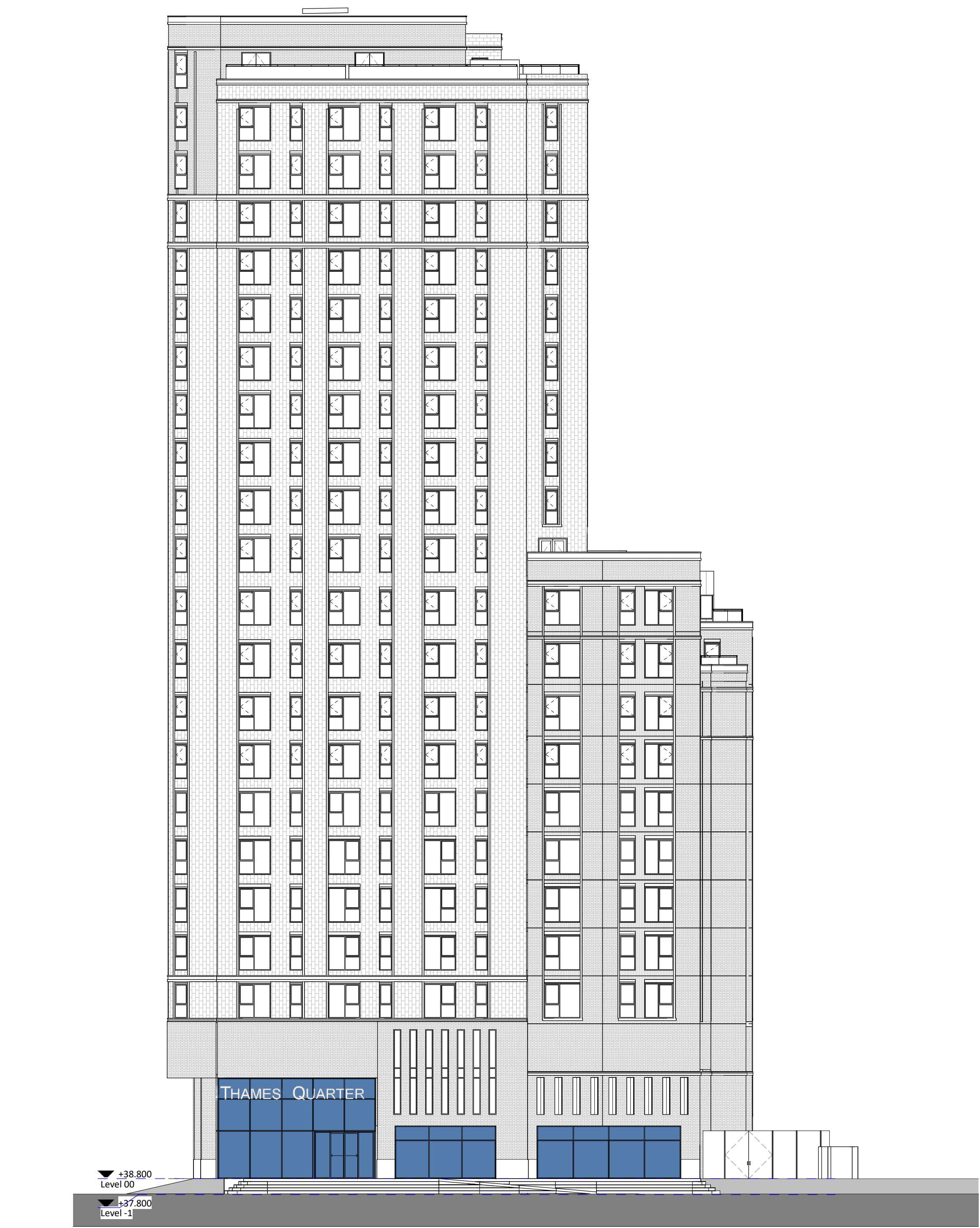
West Elevation 1 : 200
