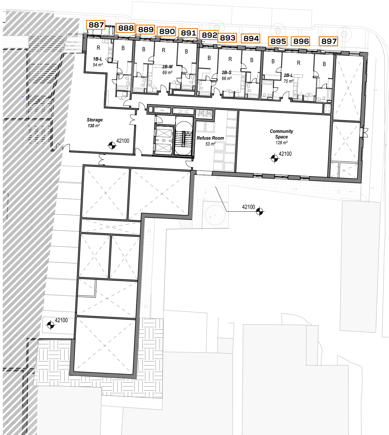
Fig. 24: Floor Plan
